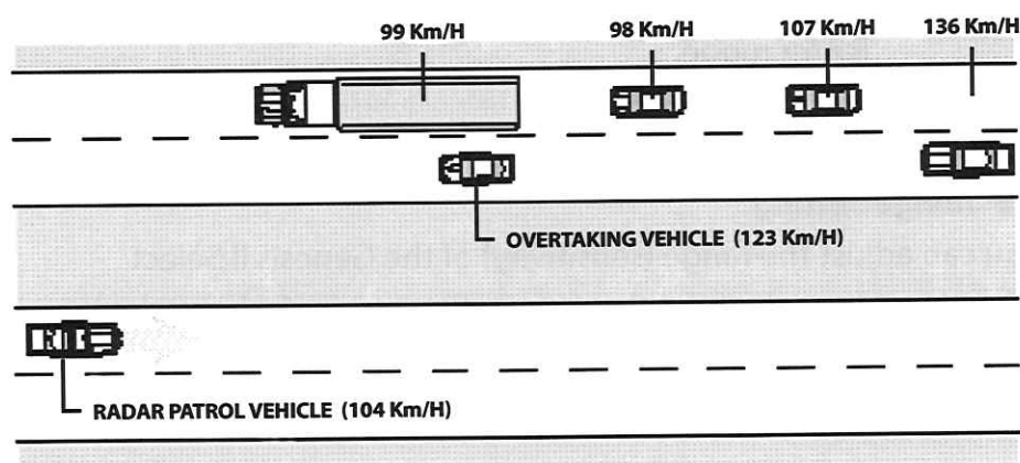
Figure 5.6 Evaluating multiple targets in Faster Mode.
