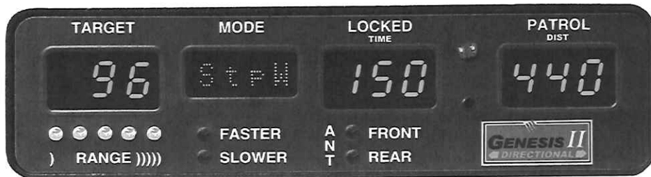
Figure 5.9 The Mode window will display "StpW" whenever the Genesis II Select is operating in the Stopwatch Mode
